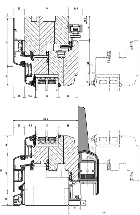
IDEALU CLASSICLINE IV 78 DETAIL VERTICAL SECTION
