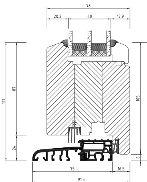
IV 78 FRENCH DOOR WITH FLAT THRESHOLD
