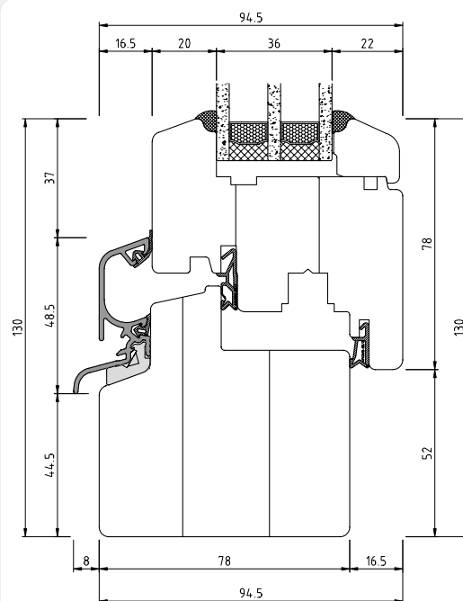
WOODEN WINDOW IV 78 PROFILE SECTION
